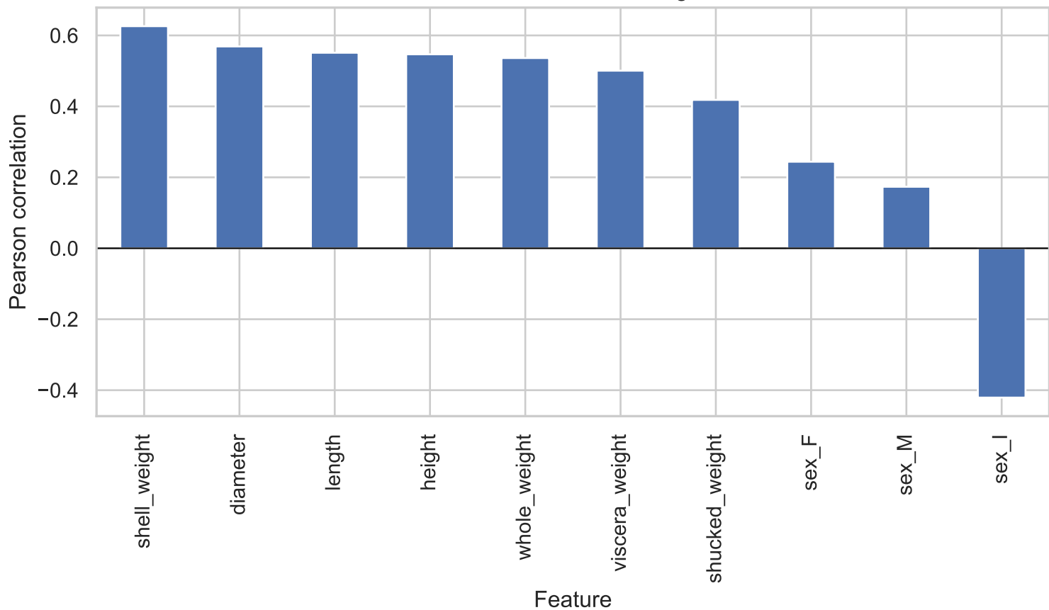
Feature correlations with ring count
