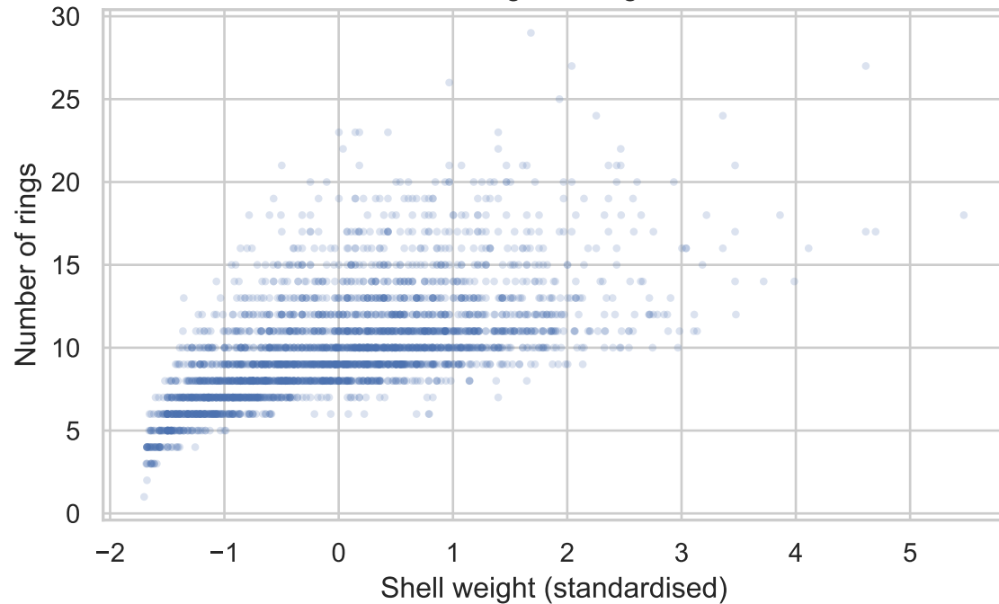
Shell weight vs ring count
