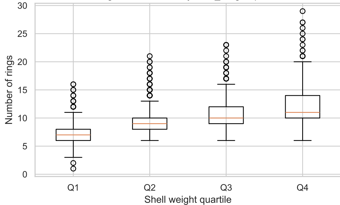
Ring count variance by shell_weight quartile
