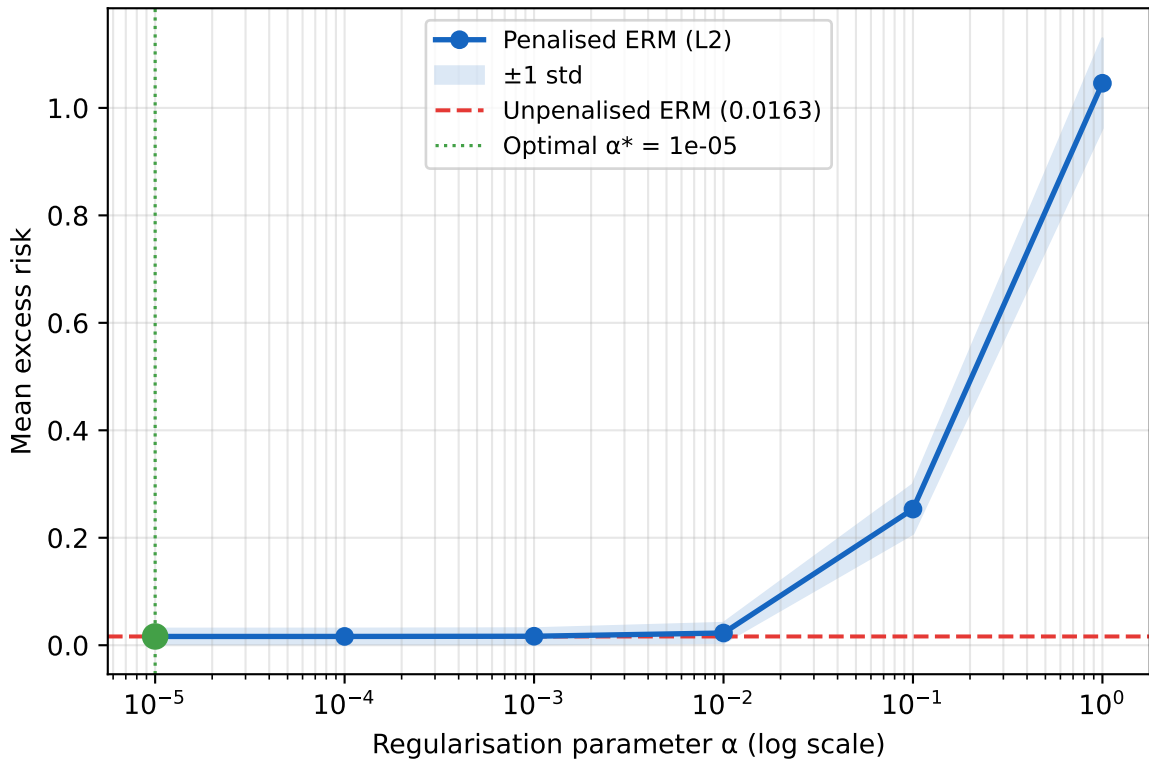
Penalty path — linear_gaussian Bias-variance tradeoff as \alpha varies
