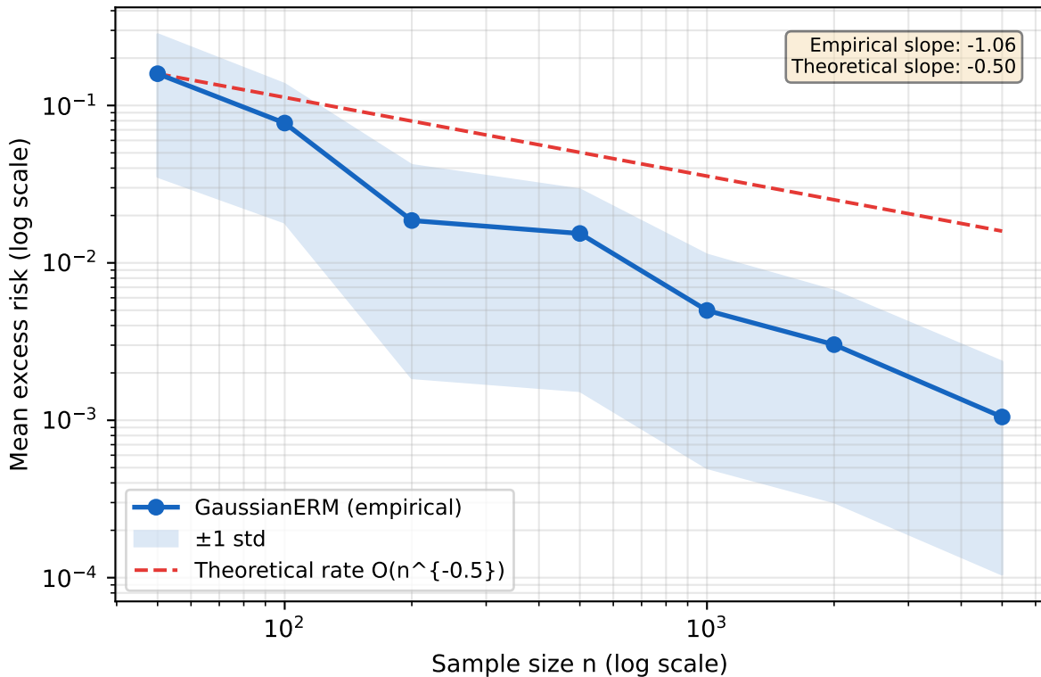
Convergence of excess risk — linear_gaussian Empirical rate vs theoretical bound
