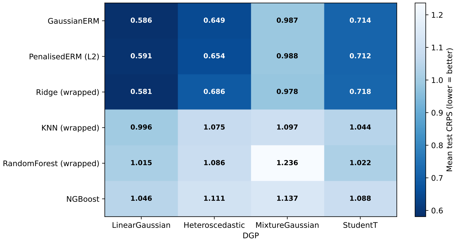
Benchmark: mean test CRPS across models and DGPs
