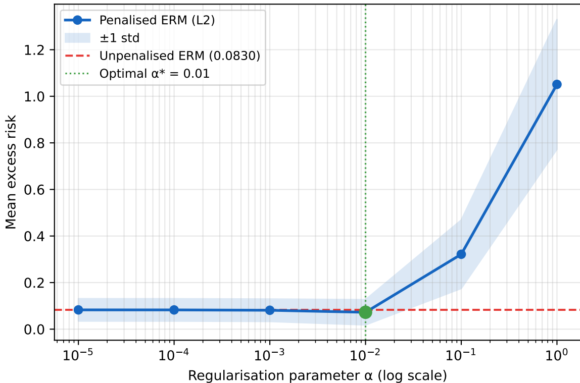
Penalty path — heteroscedastic_gaussian Bias-variance tradeoff as \alpha varies
