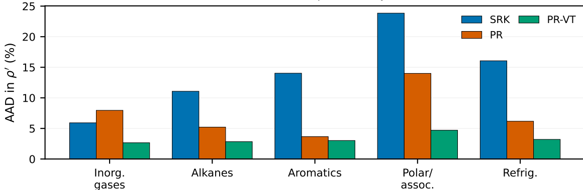
Saturated liquid density
