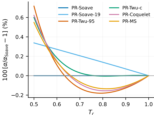
(b) PR \alpha -functions at \omega = 0.30
