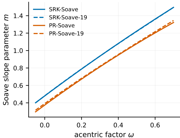
(a) m(\omega) correlations
