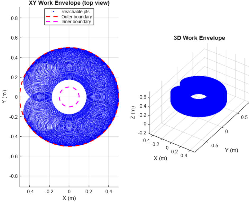
Figure 3: SCARA Work Envelope. Left: XY annular projection showing reachable points within joint limits. Right: 3D representation of the annular cylindrical workspace over the prismatic stroke.
