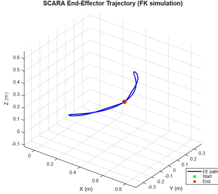
Figure 2: SCARA End-Effector Trajectory generated via Forward Kinematics (Eq. 3.8) for sinusoidal joint inputs.
