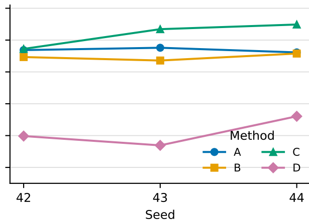
OLMo-2-1B-Instruct
