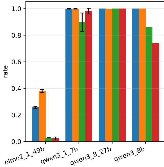
Completeness
