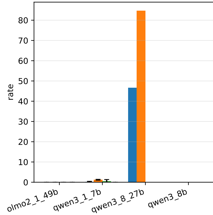
Schema validity
