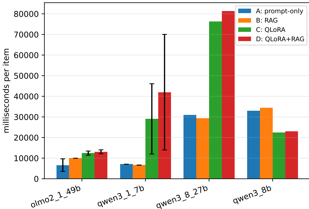
Average generation latency - dashboard_v4 Latency
