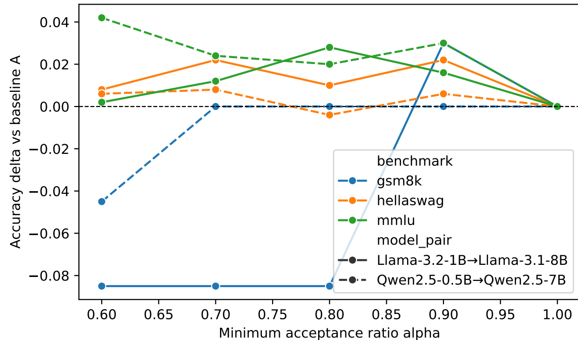
Accuracy Change vs Approximation Threshold
