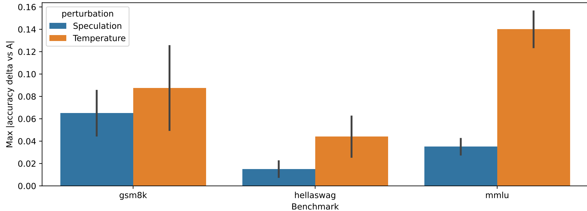
Speculative Decoding Effect Size vs Temperature Positive Control
