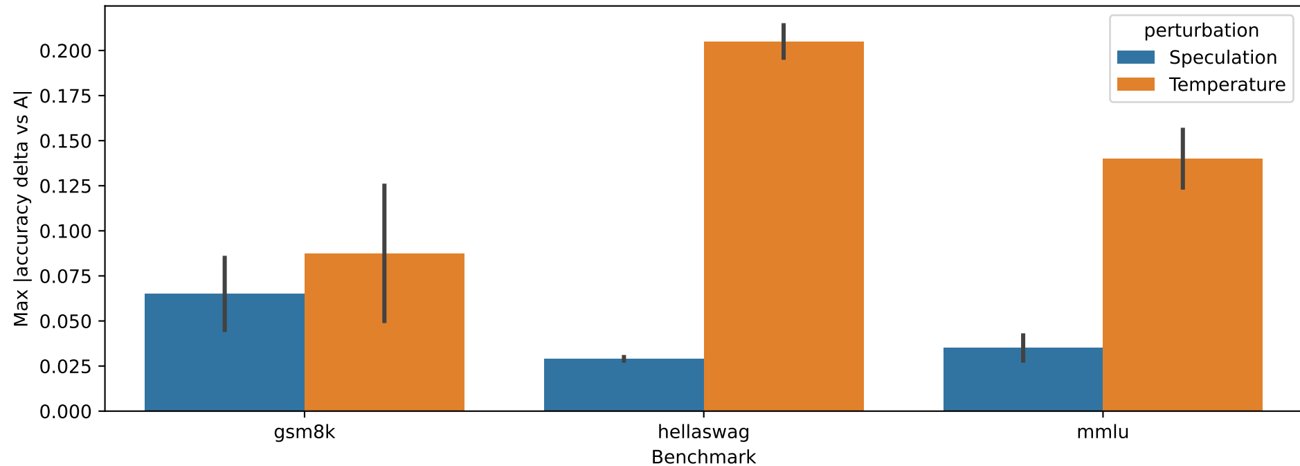
Speculative Decoding Effect Size vs Temperature Positive Control
