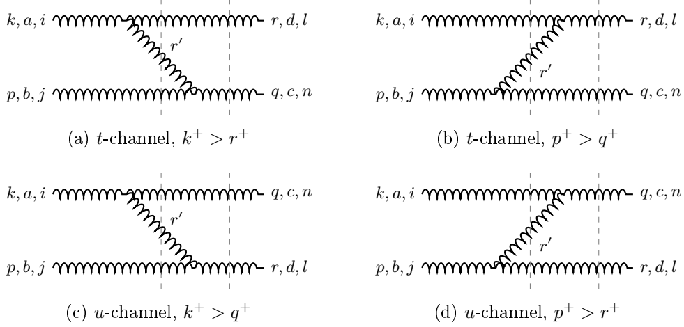
Figure 2: The light-cone time orderings of the t -channel ((a), (b)) and u -channel ((c), (d)) gluon exchange between two incoming soft gluons. The dashed vertical lines denote the intermediate (three-gluon) and final states.
