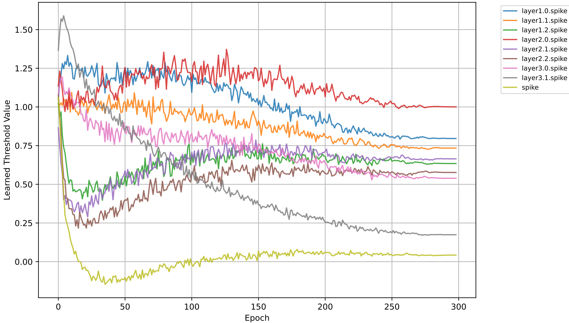
Threshold Progression Across Layers (TET-LT)
