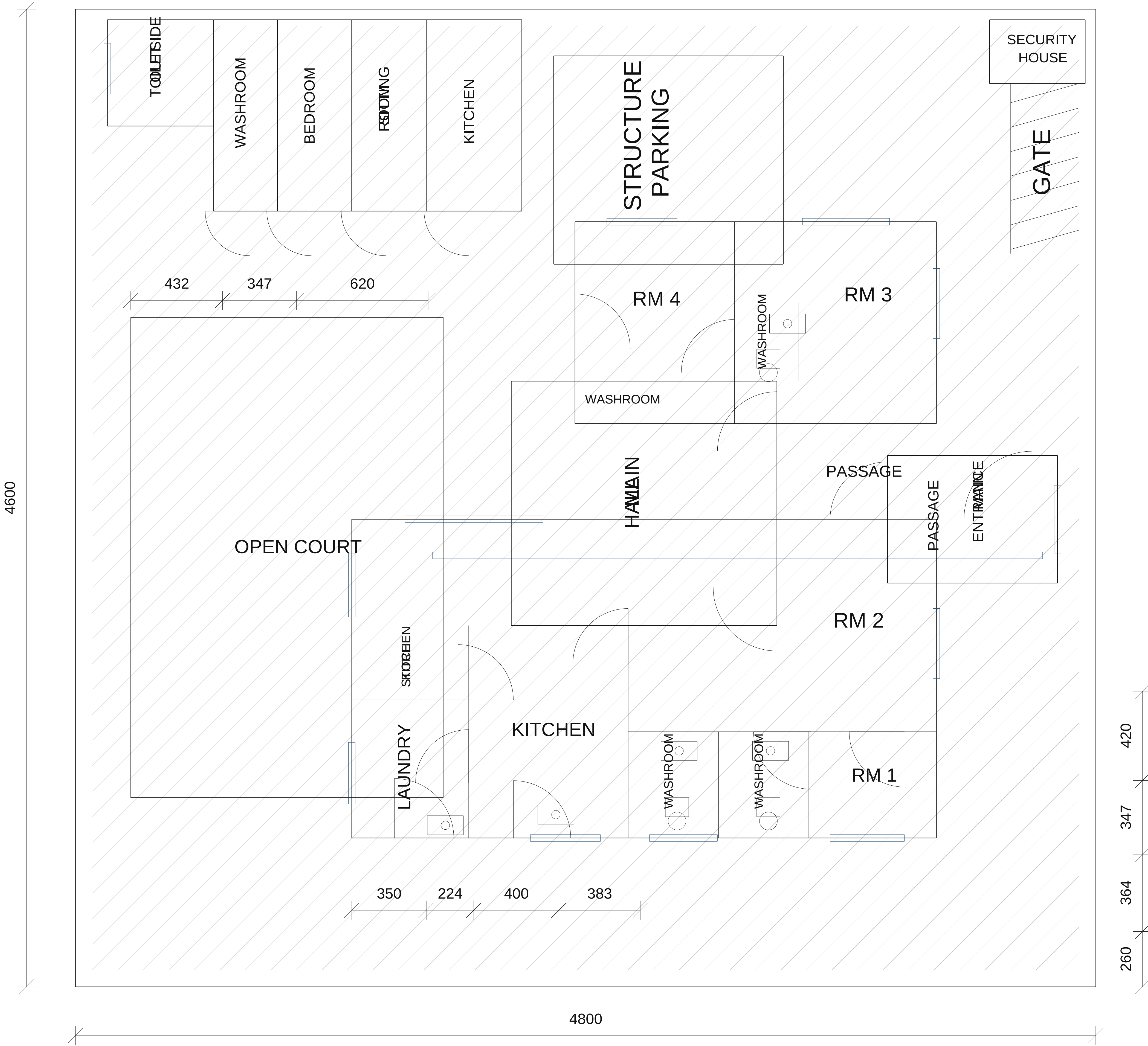
ARCHITECTURAL FLOOR PLAN FROM PROVIDED SKETCH
