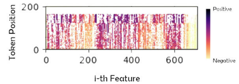
FIGURE 7. Gradient SHAP attribution scores for visual features. The x-axis represents the feature index for the OpenFace acoustic feature set, while the y-axis indicates the token position where the scores are calculated. Dark purple signifies a positive contribution to the hiring recommendation score, whereas light yellow indicates a negative contribution.
