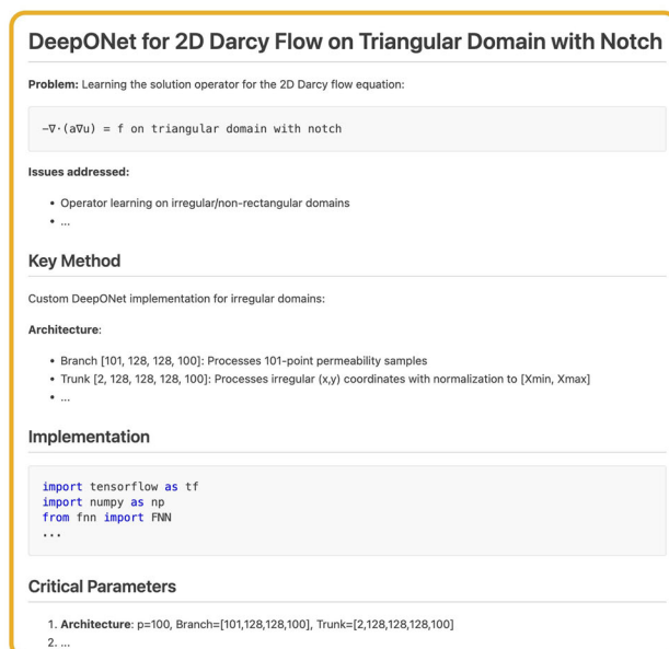
Fig. 6 | Example knowledge base entry and the JSON index summarizing method descriptions and file paths. Each KB entry is stored as a structured Markdown file containing the problem setup, issues addressed, core method, implementation code
