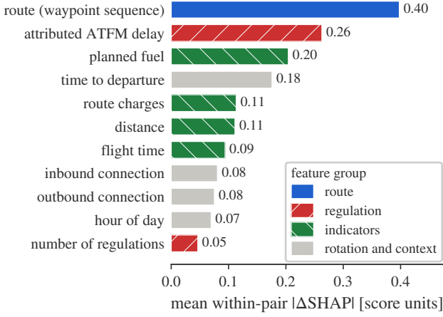
Fig. 4. What moves a decision: the mean absolute difference between a feature’s Shapley value on the two routes of a pair, over the held-out quarter, with the rotation and context groups of Table III drawn together. The waypoint sequence is the largest single term, ahead of every individual cost indicator, though the four taken together sum to more; attributed ATFM delay outweighs planned fuel. Shared context features affect the comparison through interactions; outbound connection time can also differ between routes.
