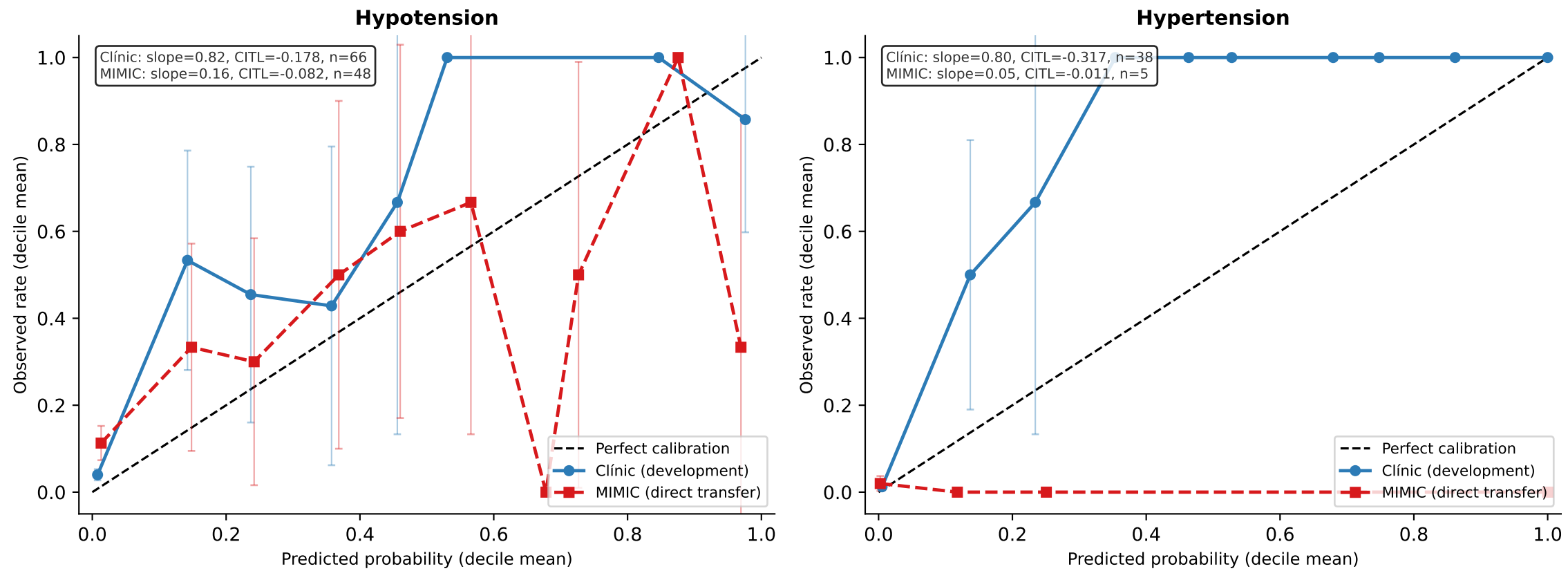
Fig. 7 — GLMM model calibration: predicted vs observed probability Intraoperative hypotension and hypertension
