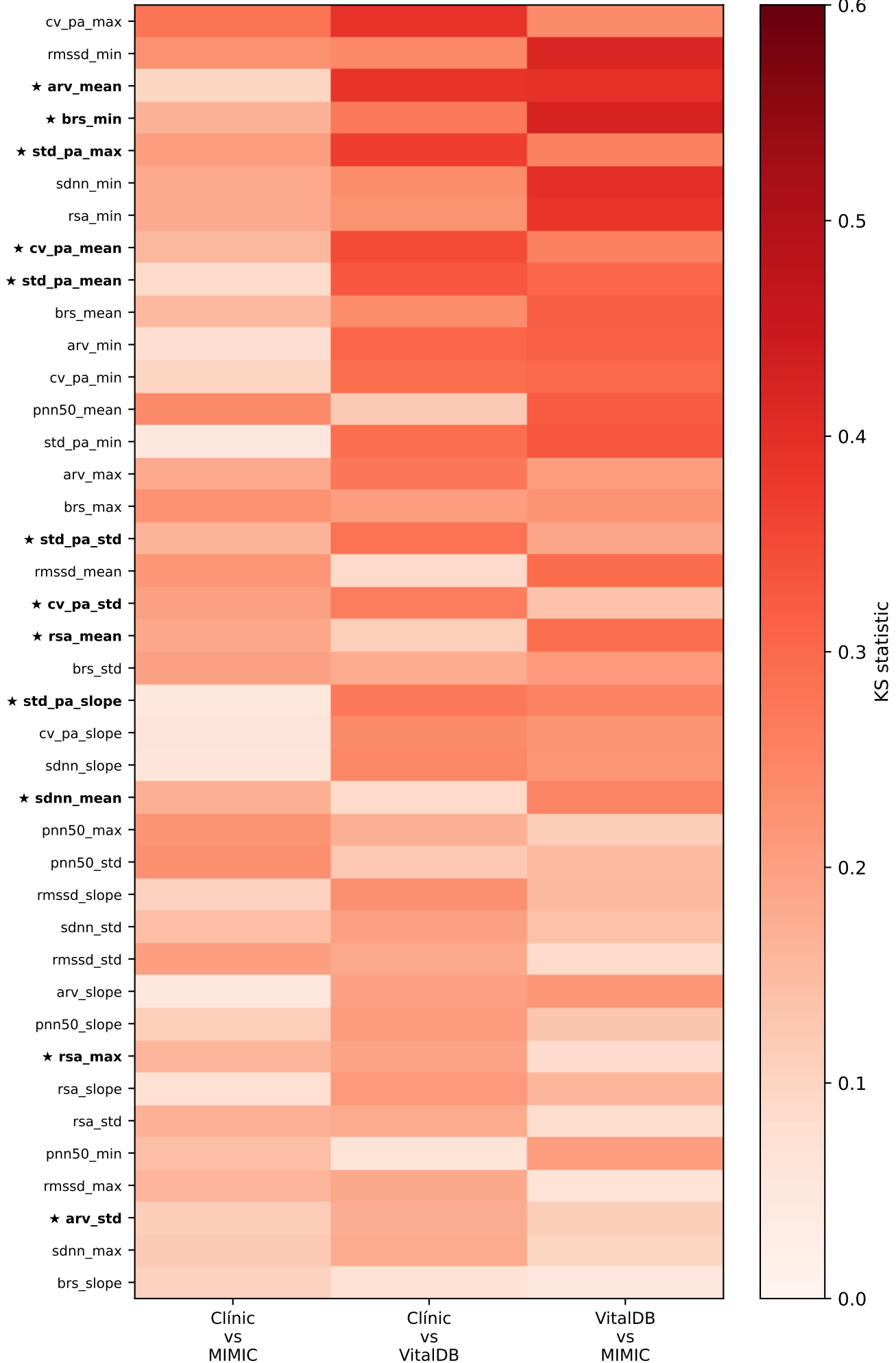
Feature Distribution Shift (KS statistic)
