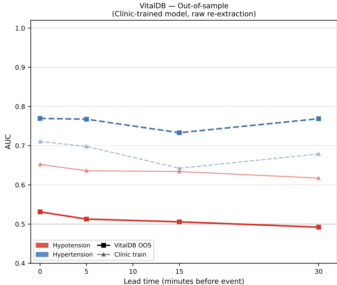
Fig 4 — Temporal persistence of prediction performance (0-30 min lead time)
