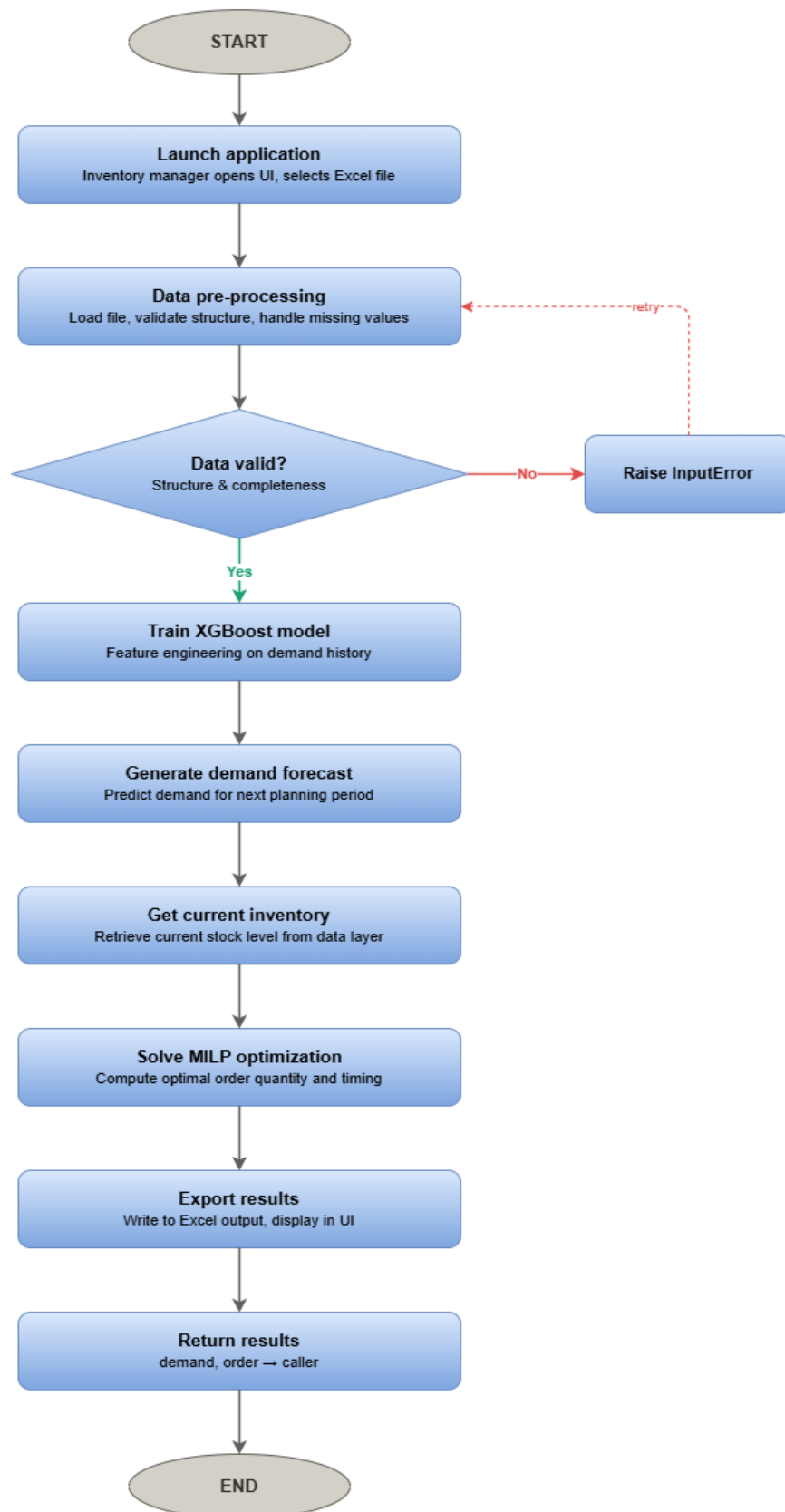
Figure 9: Flowchart
