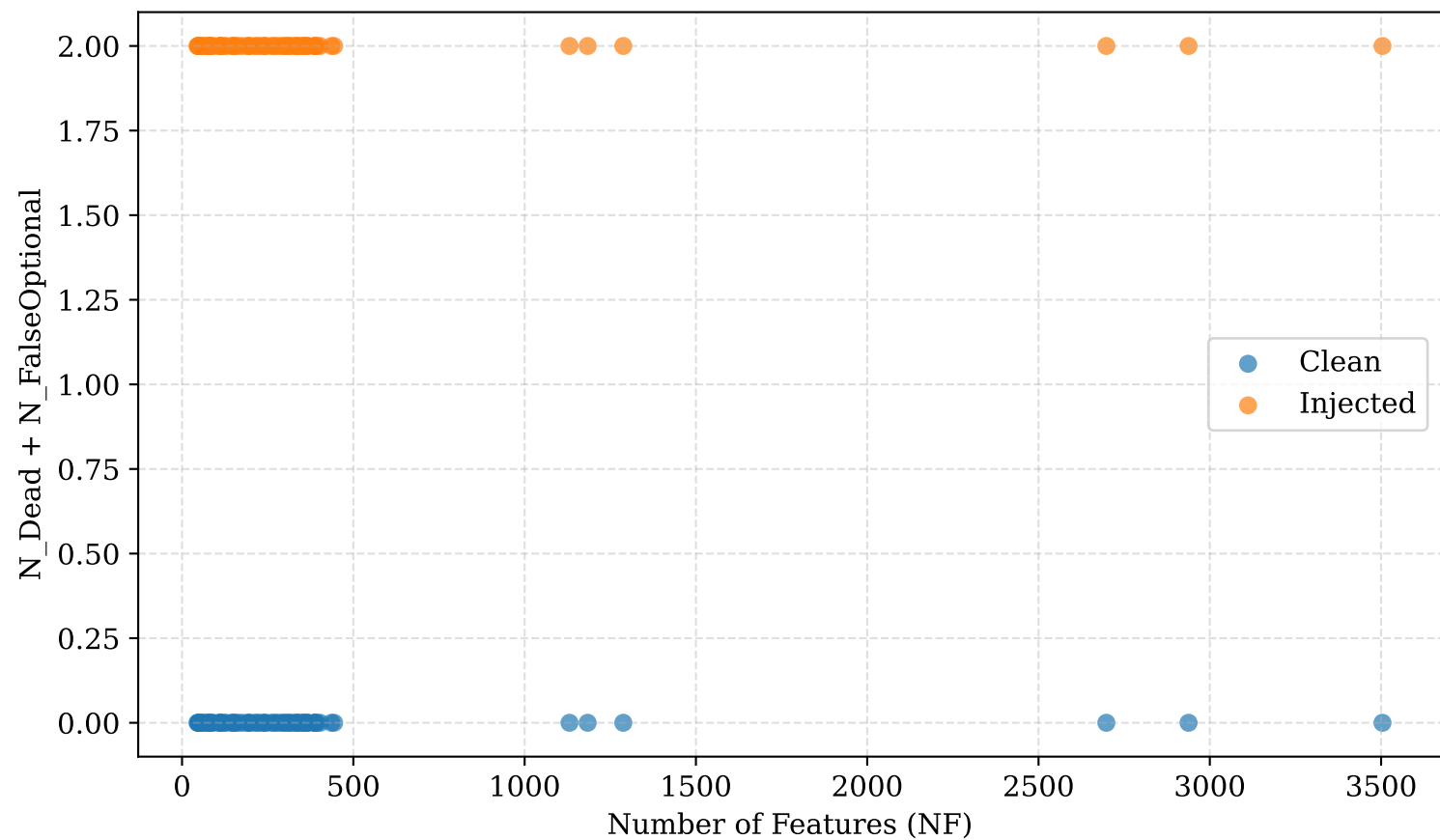
Detected Defects Count vs Model Size
