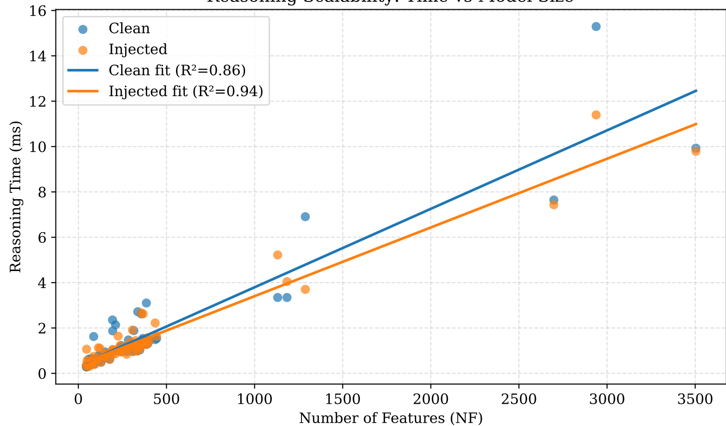
Reasoning Scalability: Time vs Model Size
