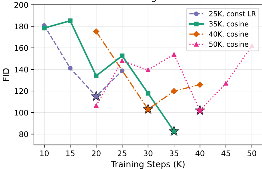
Schedule Length Ablation
