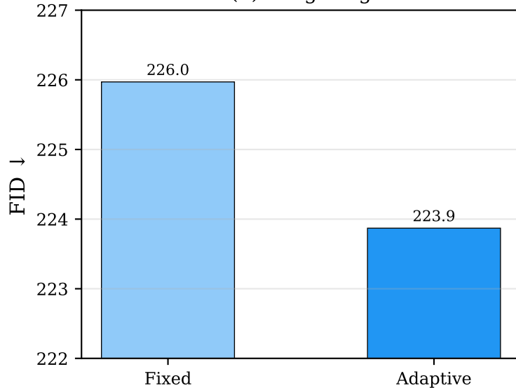
(b) Weighting
