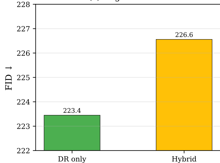
(c) Regularization
