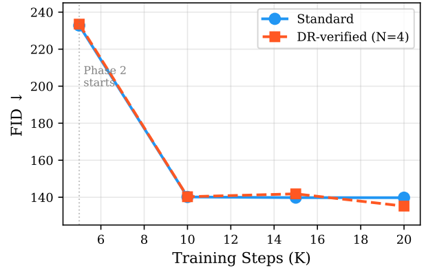
Figure 2. FID trajectory during training. Phase 2 (DM + regression) begins at 5K steps, producing a sharp FID drop from 233 to 140 within the next 5K steps. DR-4 verification provides an additional 4.6-point improvement at 20K steps.
