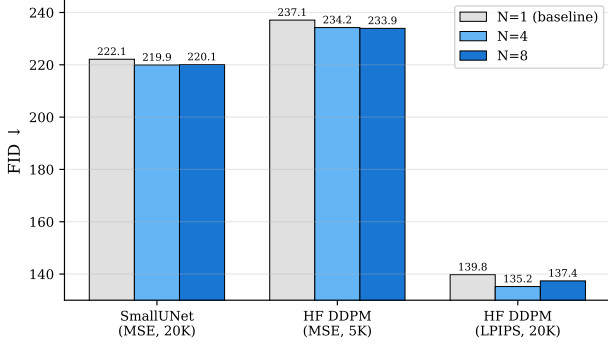
Figure 3. Density-ratio verification (best-of- N ) improves FID. For the extended LPIPS model, DR-4 provides a 4.6-point improvement.
