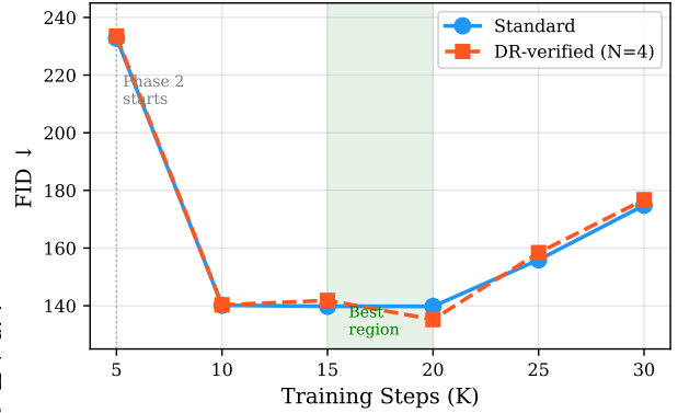
Figure 2. FID trajectory during training. Phase 2 (DM + regression) begins at 5K steps, producing a sharp FID drop from 233 to 140. Quality peaks at 15–20K steps and degrades beyond 20K as the regression weight decays, indicating the LPIPS anchor is essential throughout training.
