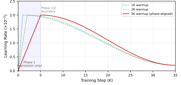
Figure 6. Learning rate schedules for three warmup durations. With 5K warmup (phase-aligned), the LR peaks at the Phase 1/Phase 2 boundary and immediately decays. Shorter warmup causes the LR to peak during Phase 1 and partially decay before the DM loss activates.
