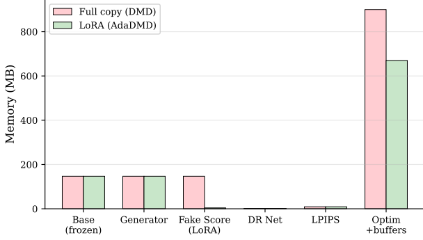
Figure 7. Memory breakdown: LoRA (AdaDMD) vs. full copy (DMD). The fake score model shrinks from 147 MB to 4 MB.
