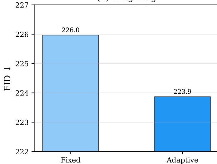
(b) Weighting
