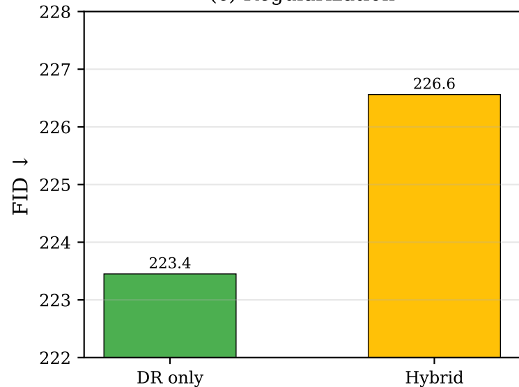
(c) Regularization
