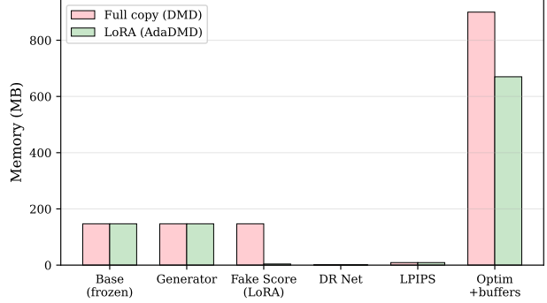
Figure 6. Memory breakdown: LoRA (AdaDMD) vs. full copy (DMD). The fake score model shrinks from 147 MB to 4 MB.
