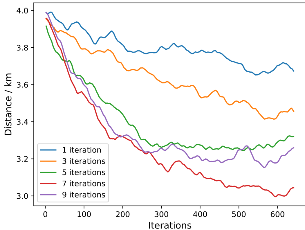
Different Fine-tune interval
