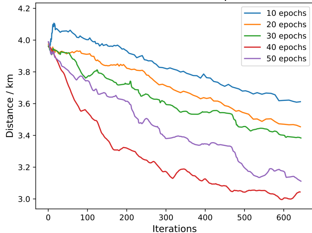
Different Fine-tune Epoch
