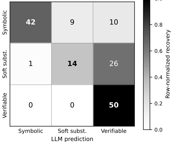
GPT-5.5 \kappa = 0.54 , 69.7% agree ( n = 152 )
