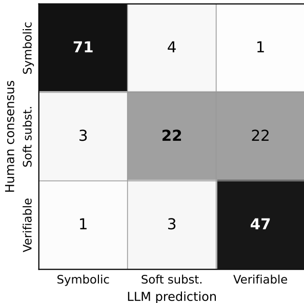
Claude Sonnet 4.5 \kappa = 0.70 , 80.5% agree ( n = 174 )
