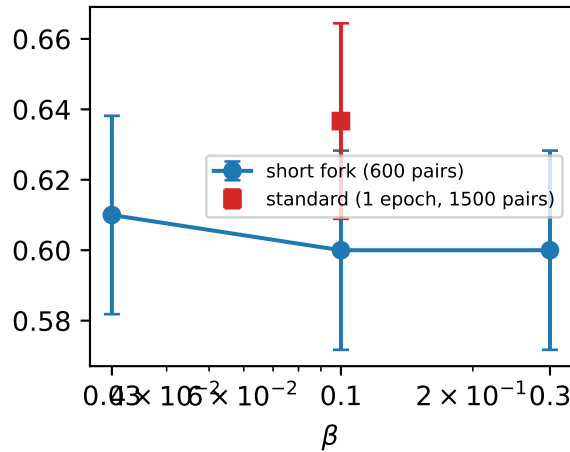
Held-out pref. accuracy
