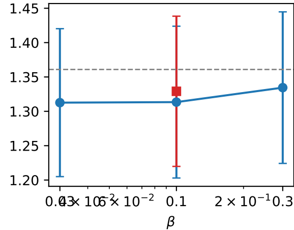
RM score
