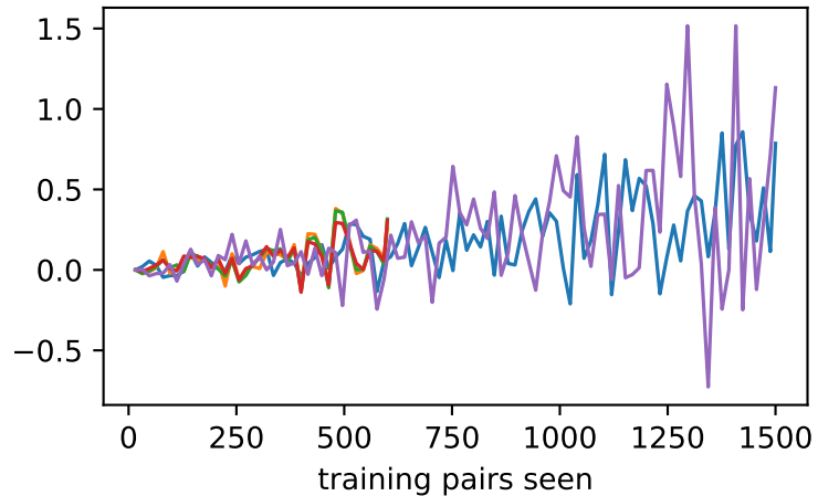
train margin_mean
