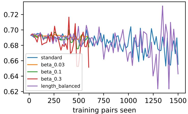
train loss
