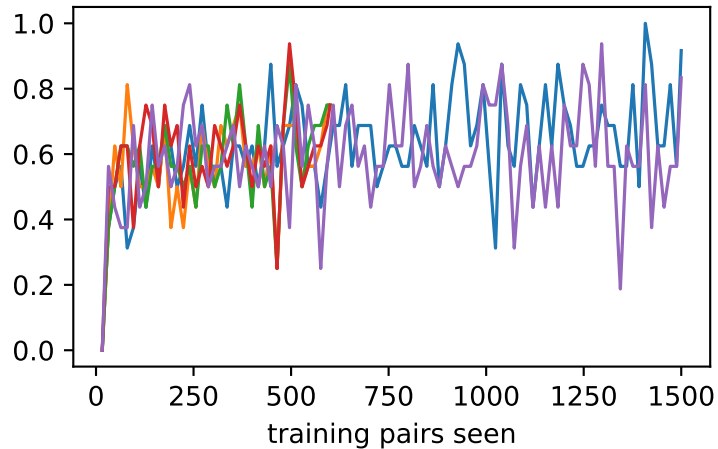
train preference_accuracy
