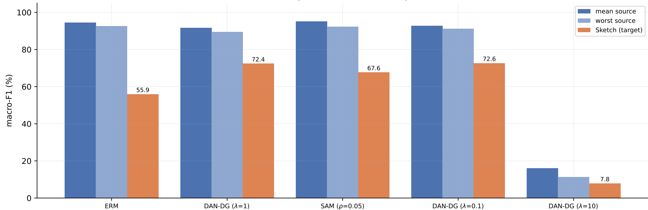
Source validation performance does not predict Sketch
