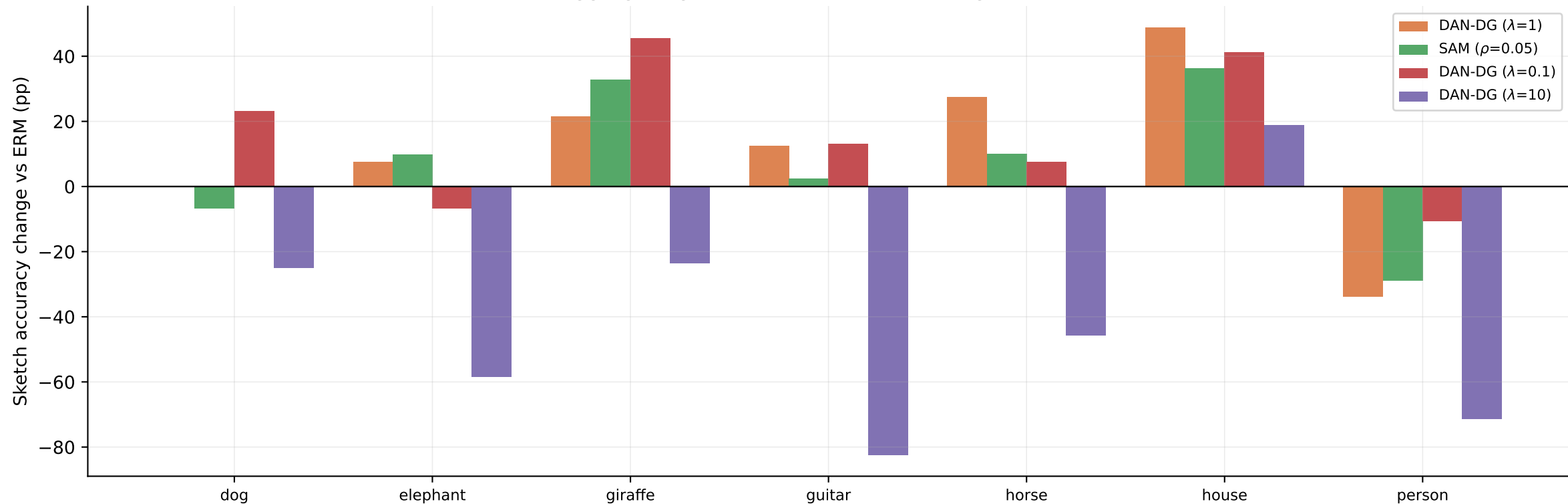
An aggregate gain can hide class-level negative transfer
