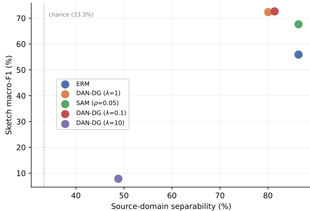
(a) Source invariance vs transfer
