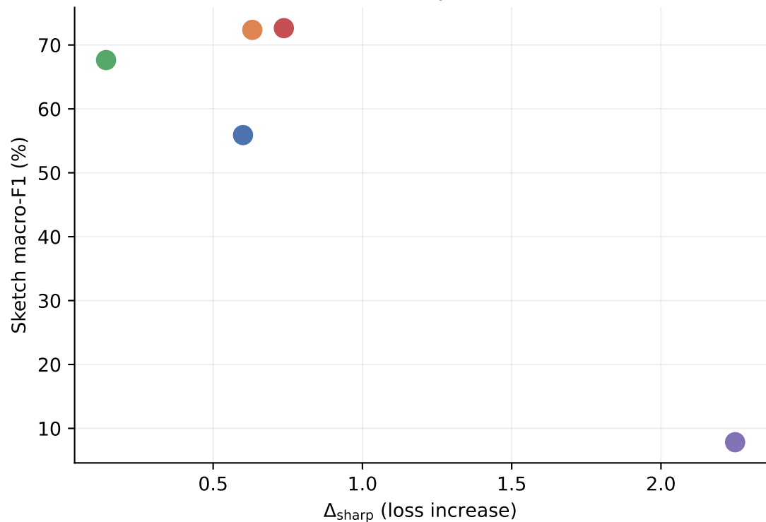
(b) Local stability vs transfer
