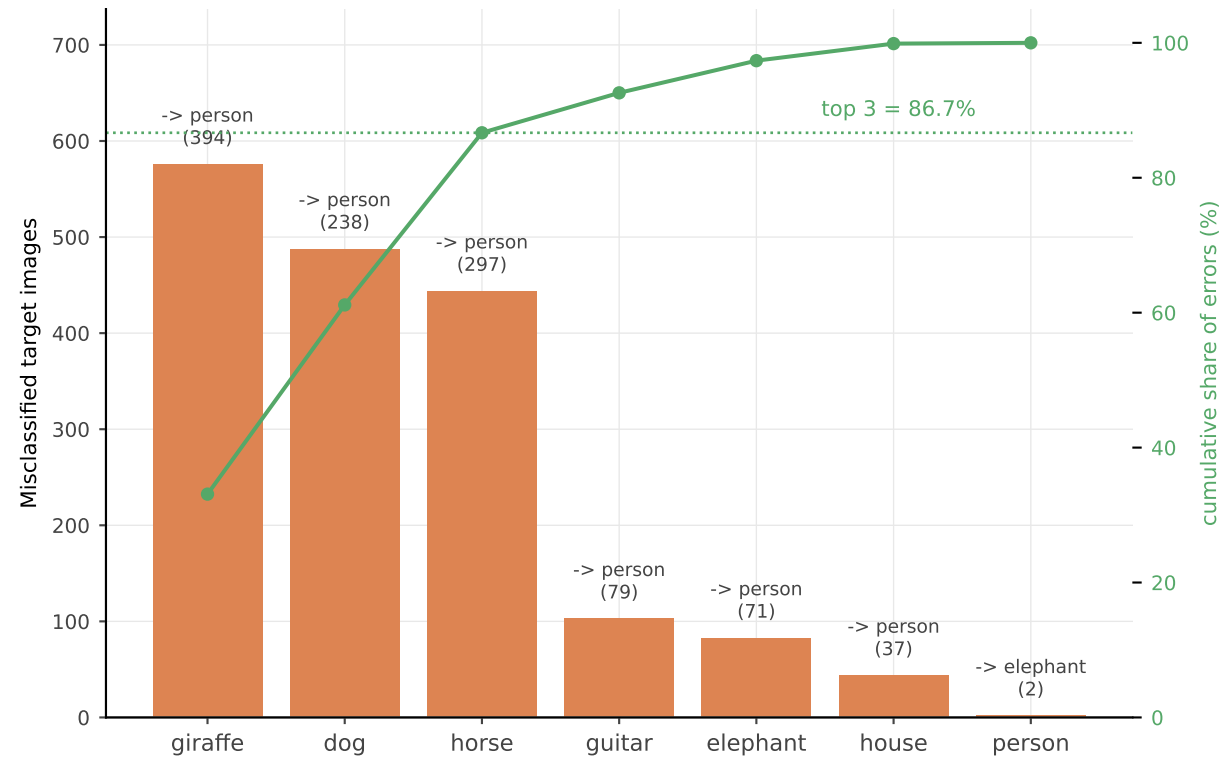
(b) Error contribution and dominant confusion
