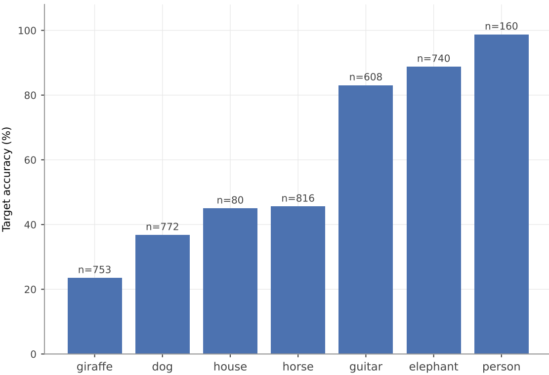
(a) Source-only ERM, per class on Sketch
