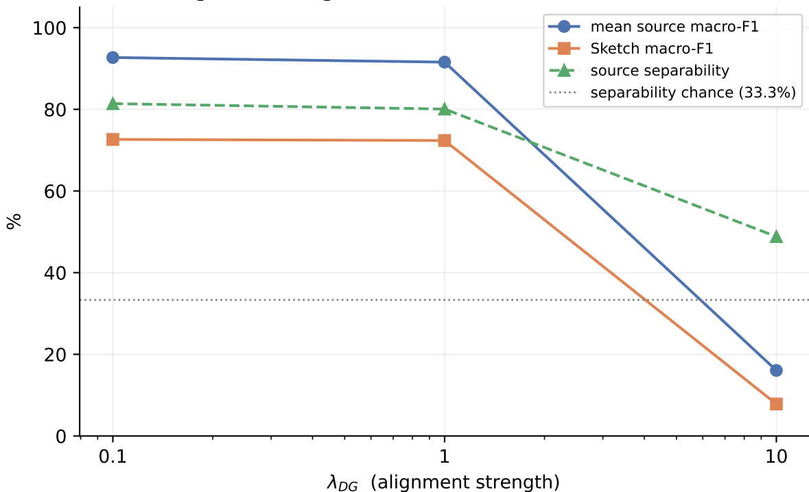
Increasing source alignment: too much removes class structure
