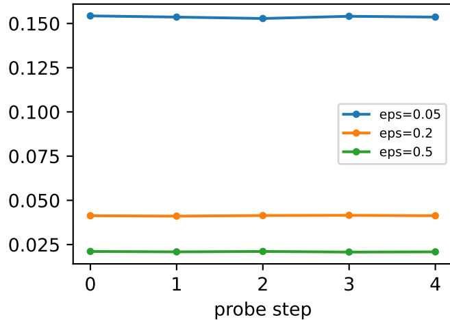
clip fraction (cached batch)
