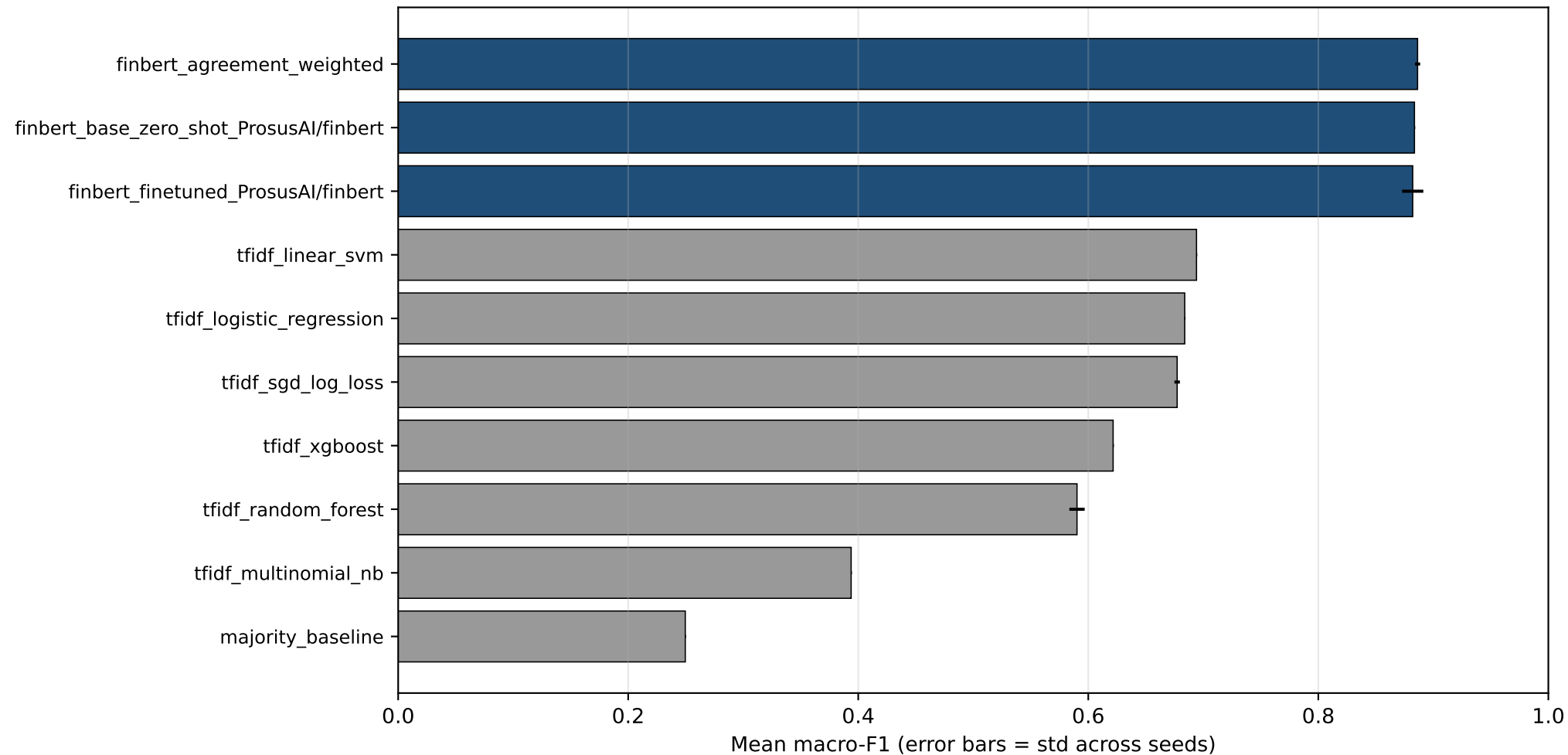
CARA-FinSent — Macro-F1 leaderboard (PhraseBank, in-domain)
