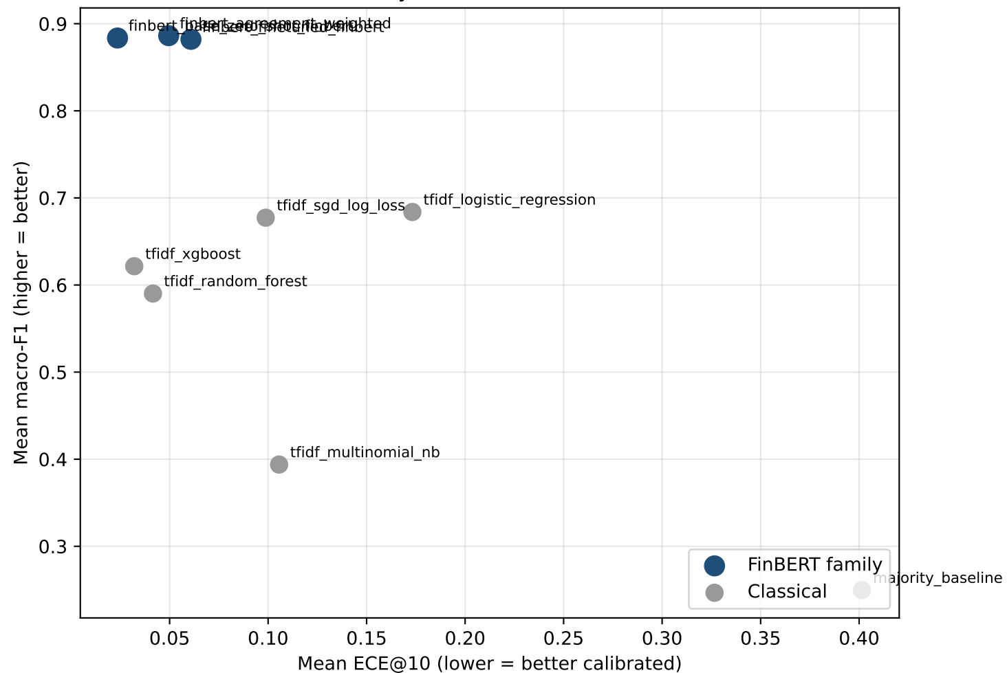
Accuracy vs calibration trade-off
