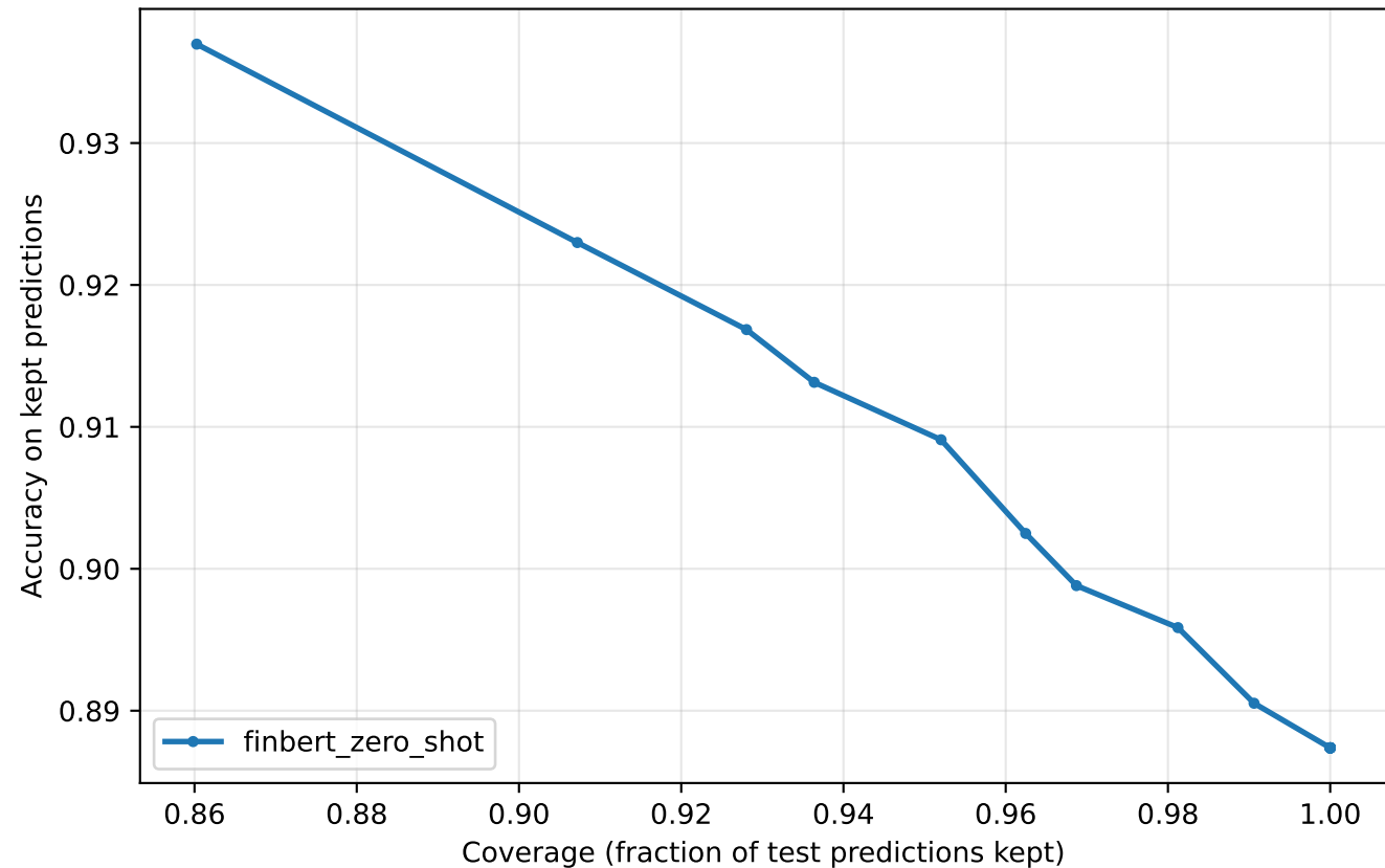
Abstention trade-off: coverage vs accuracy
