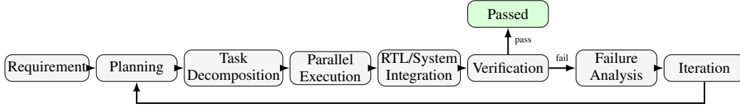
Figure 1. The MACE pipeline. Verification gates every integrated change against Verilator simulation. The run ends when every gate workload passes; any failure triggers failure analysis and a replan.
