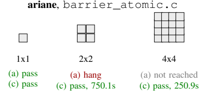
Figure 2. Left: all three cores, same 1x1 objective. (b) never passes. On sparc/pico, (c) exhausts its retry budget instead of reporting a false pass; only arianes passes , under (c). Right: manual mesh scaling (a) vs. (c), arianes only. Green =pass, red =hang, gray =not reached. The loop passes both shapes (a) got stuck on.
