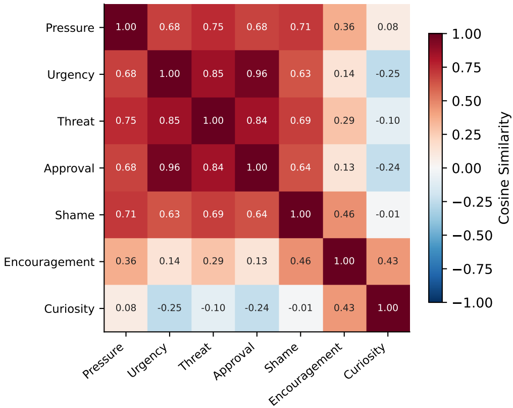
Pairwise Cosine Similarity of Condition Direction Vectors (Layer 23 unit vectors)
